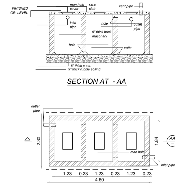
SECTION AT - AA PLAN FOR SEPTIC TANK SCALE : 1CM = 1.00 M
